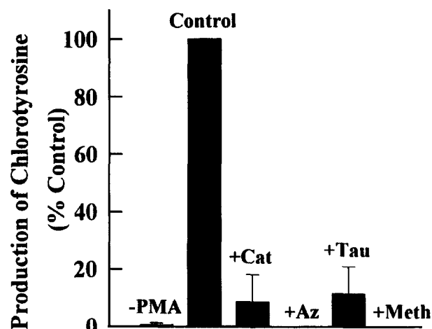
Fig. 5. Effect of inhibitors on the chlorination of albumin by neutrophils. Neutrophils were incubated with 500 \mu\text{g/ml} of albumin and stimulated with phorbol myristate acetate (PMA) for 30 min in the absence (control) or presence of 50 \mu\text{g/ml} of catalase (Cat), 1 mM azide (Az), 10 mM taurine (Tau), or 1 mM methionine (Meth). Reaction conditions and determination of chlorotyrosine are described in section 2. Results are expressed as means and standard deviations of four separate experiments.
